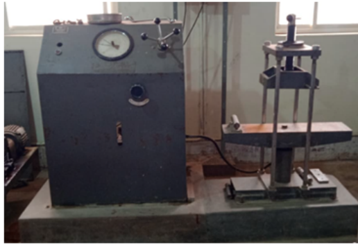
Flexural testing machine set up
